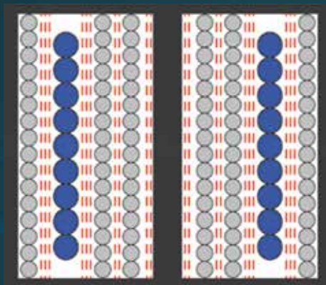
Figure 1 - Standard Transformer section structures
